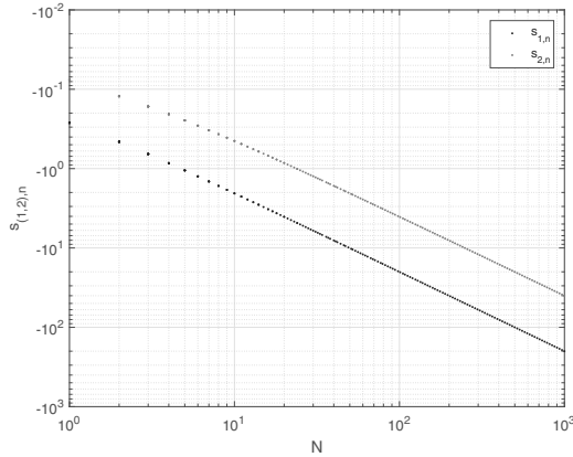
Fig. 5. Logarithmic plot of eigenvalues s_{(1,2),n} of the section state matrix A_n vs. the number of sections N .
