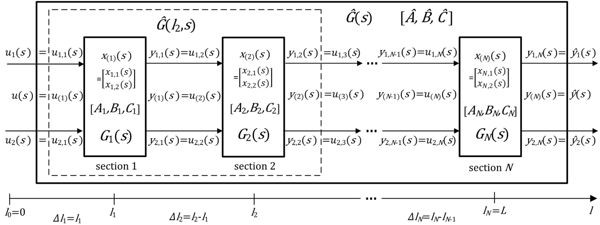
Fig. 3. Block diagram of the approximation state space and transfer function models.
