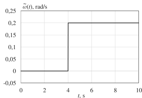
Fig. 6. Estimate of the function \tilde{\omega}(t) .
