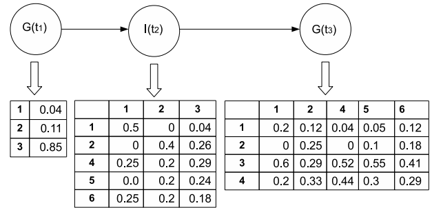
Fig. 4. Example Bayesian network.
