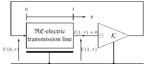
Fig. 4. Proportional feedback control of an \Re\mathfrak{C} transmission line.
