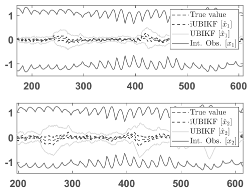
Fig. 7. Estimation results for the UBIKF, the iUBKF and the interval observer for the two-wheeled vehicle model: the angular speed of the slideslip angle x_1 (top) and the acceleration of the vehicle yaw x_2 (bottom).
