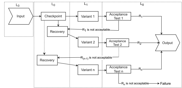
Fig. 6. Basic iRB configuration, employing n variants and 2 protection layers.
