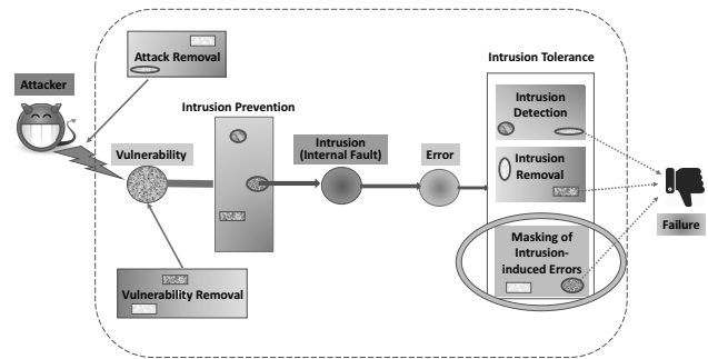
Fig. 1. Representation of the attack-vulnerability-intrusion-error-failure chain (inspired by Veríssimo et al. (2003)) and technique categories to cope with it.
