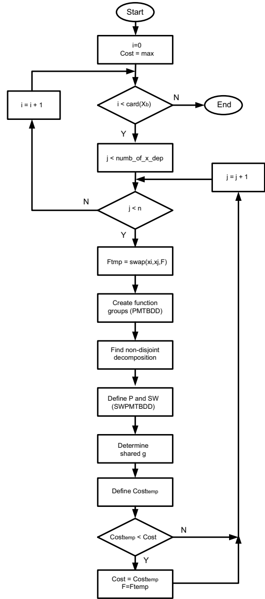
Fig. 9. Decomposition algorithm aimed at minimizing dynamic power.
