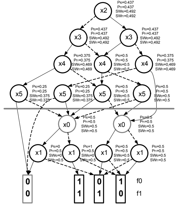
Fig. 6. SWMTBDD example.
