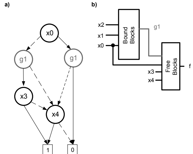
Fig. 2. Non-disjoint decomposition: BDD in which g_0 is replaced by x_0 (a), partition model for non-disjoint decomposition (b).
