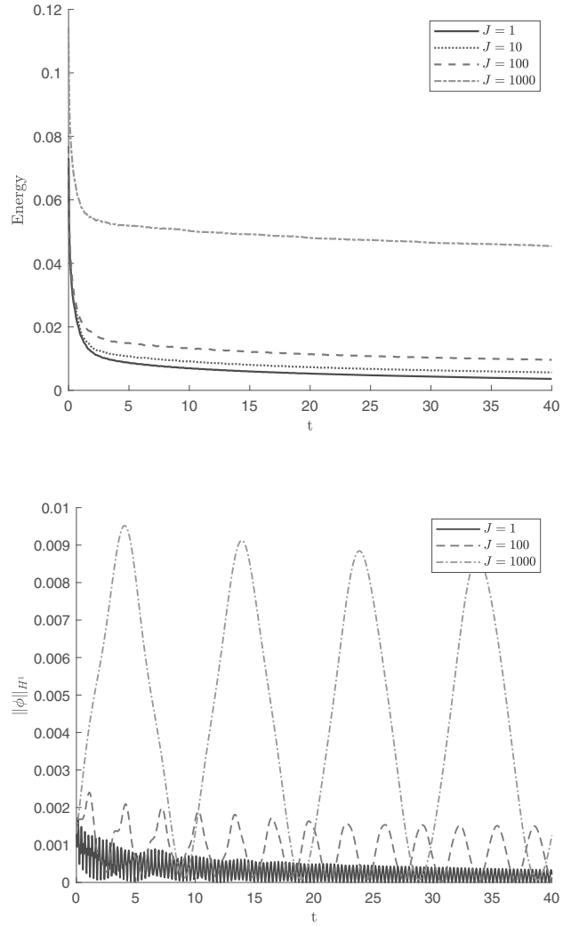
Fig. 3. Different behaviours of the discrete energy (top) and the solution (bottom) depending on J .
