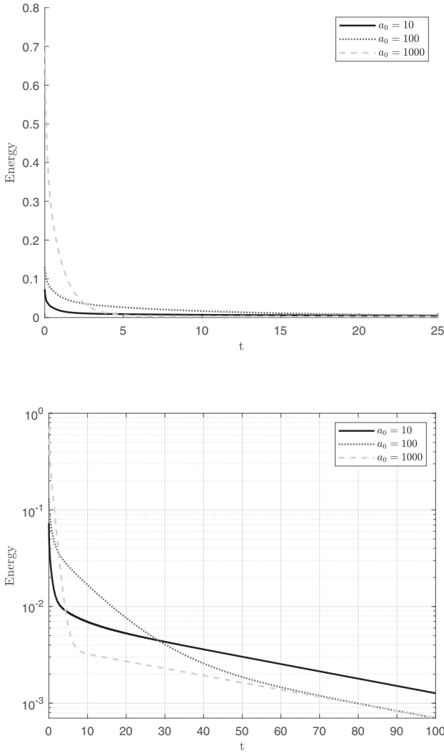
Fig. 2. Exponential decay of the energy for different values of a_0 .
