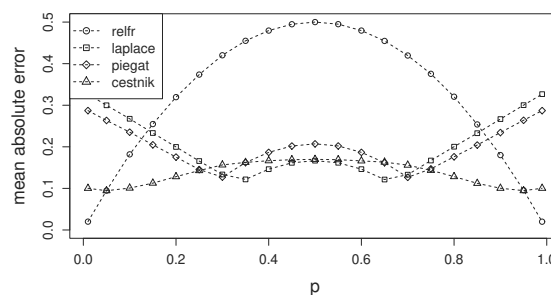
Fig. 6. Comparison of MAEs of the four estimation methods, p_d distortion of p_a for the m -estimate = 0.3.
