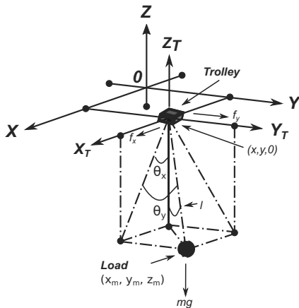
Fig. 1. Overhead crane.
