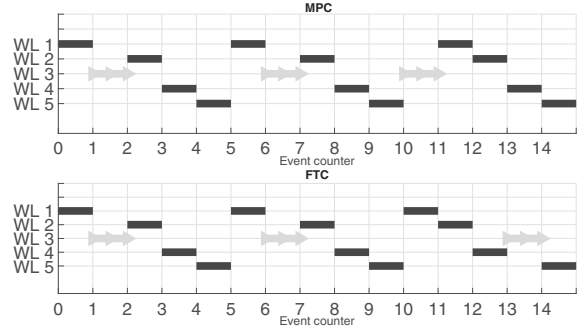
Fig. 10. Scheduling scheme for the fault-free scenario.
