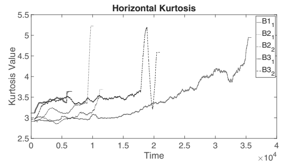
Fig. 6. Kurtosis of vibration signals.
