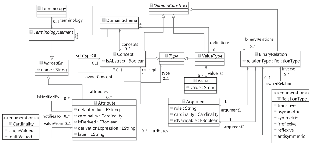
Fig. 4. Excerpt from the CML metamodel: concept and relationship.
