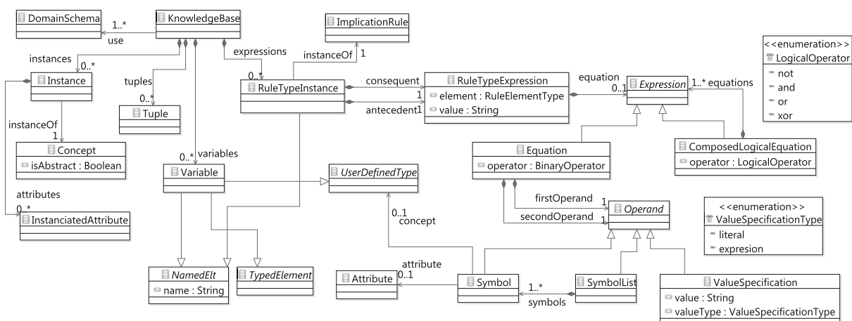
Fig. 6. Excerpt from the CML metamodel: knowledge base and rule type instance.
