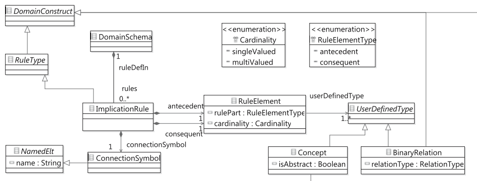
Fig. 5. Excerpt from the CML metamodel: rule type.
