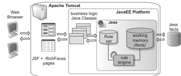
Fig. 10. Rule-based Web application architecture.
