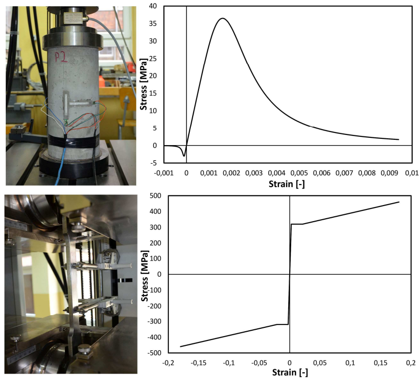
Fig. 3. Physical laws of materials
