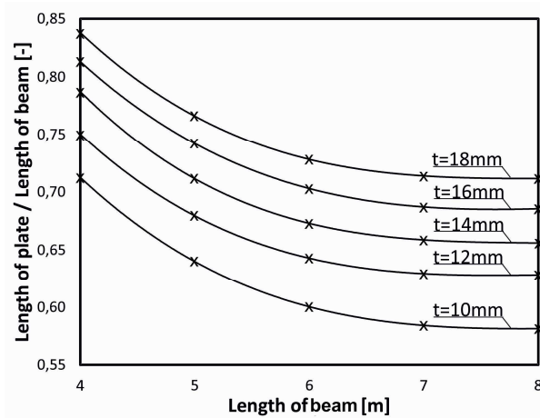
Fig. 11. Curves of the desired length of the plate depending on its thickness
