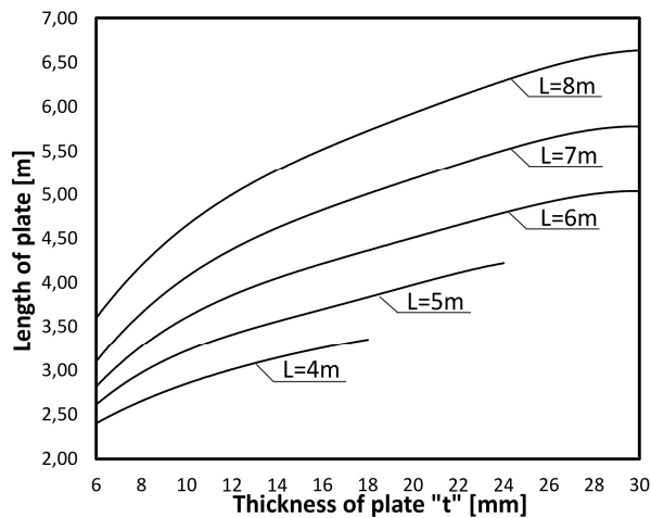
Fig. 9. Optimal dimensions of the strengthening plate for different lengths of the beam
