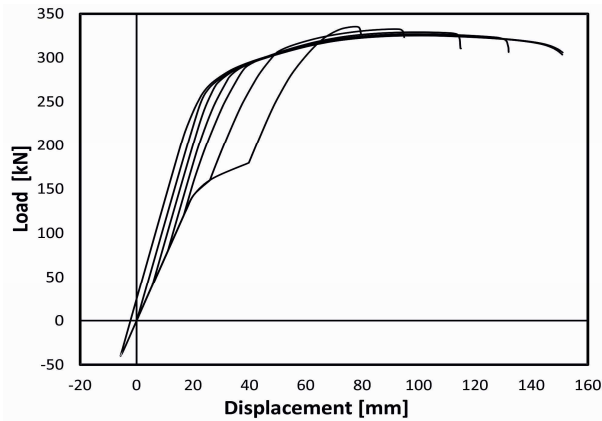
Fig. 6. Static equilibrium paths for different load levels during strengthening
