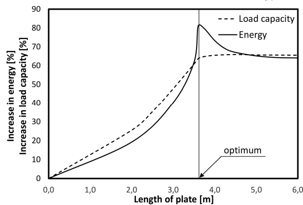
Fig. 7. Variation of energy and load capacity for a 6 metre-long beam strengthened with plates of different lengths
