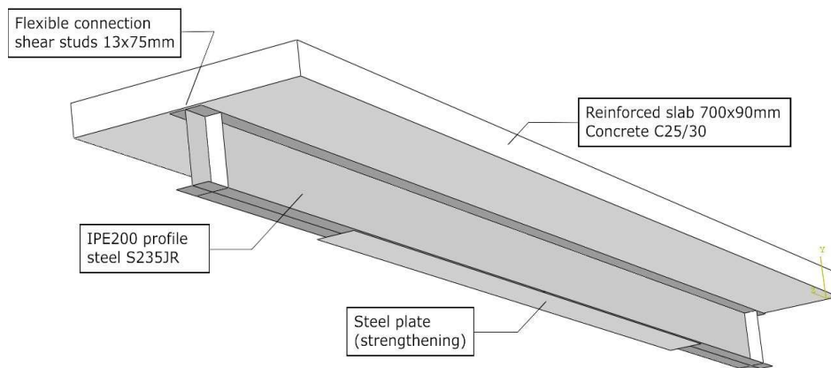
Fig. 1. General view of the analysed model
