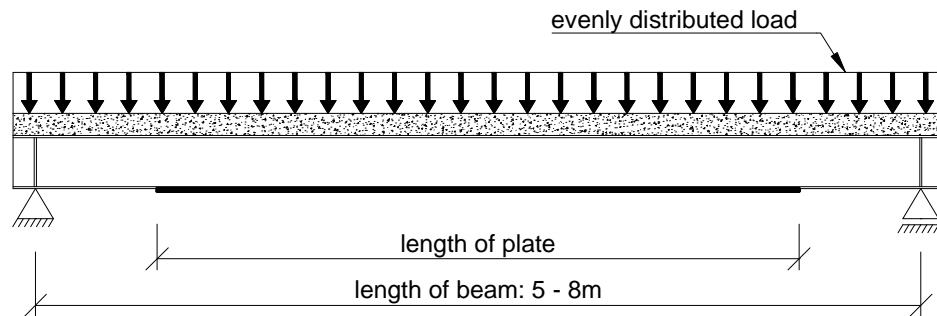
Fig. 5. The static scheme of the analysed beams
