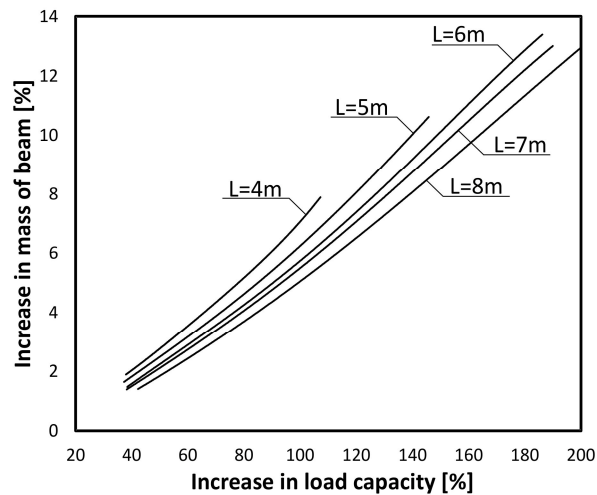
Fig. 12. Relation between the increase in the load-bearing capacity and the increase in the mass of the strengthened beam
