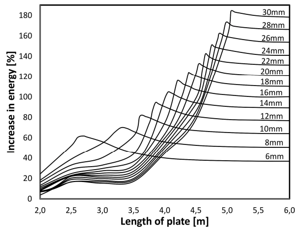
Fig. 8. Energy increase against the length of the plate for various thicknesses of the plate
