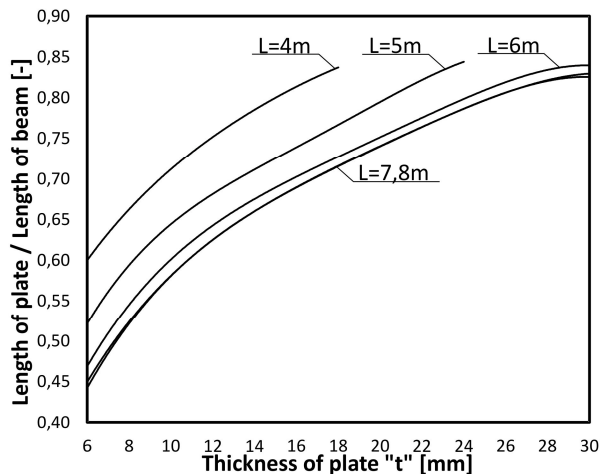
Fig. 10. Optimal dimensions of the strengthening plate for different lengths of the beam
