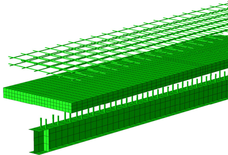
Fig. 4. Discrete model of the composite beam
