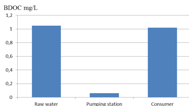
Fig. 4. Changes in BDOC contents during the treatment and distribution of water
