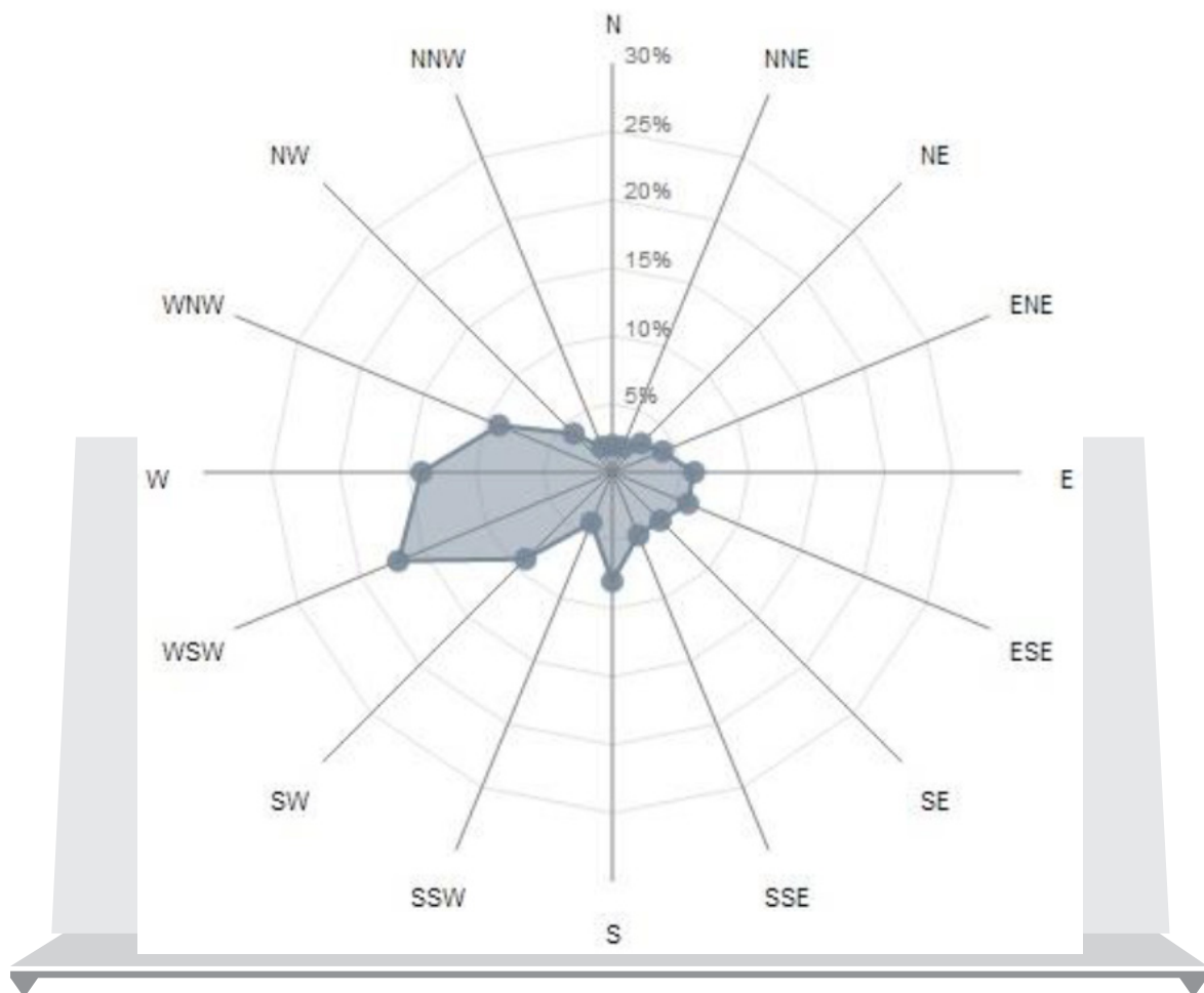
Figure 4. The distribution of wind directions [%] in Zielona Gora in 2015
