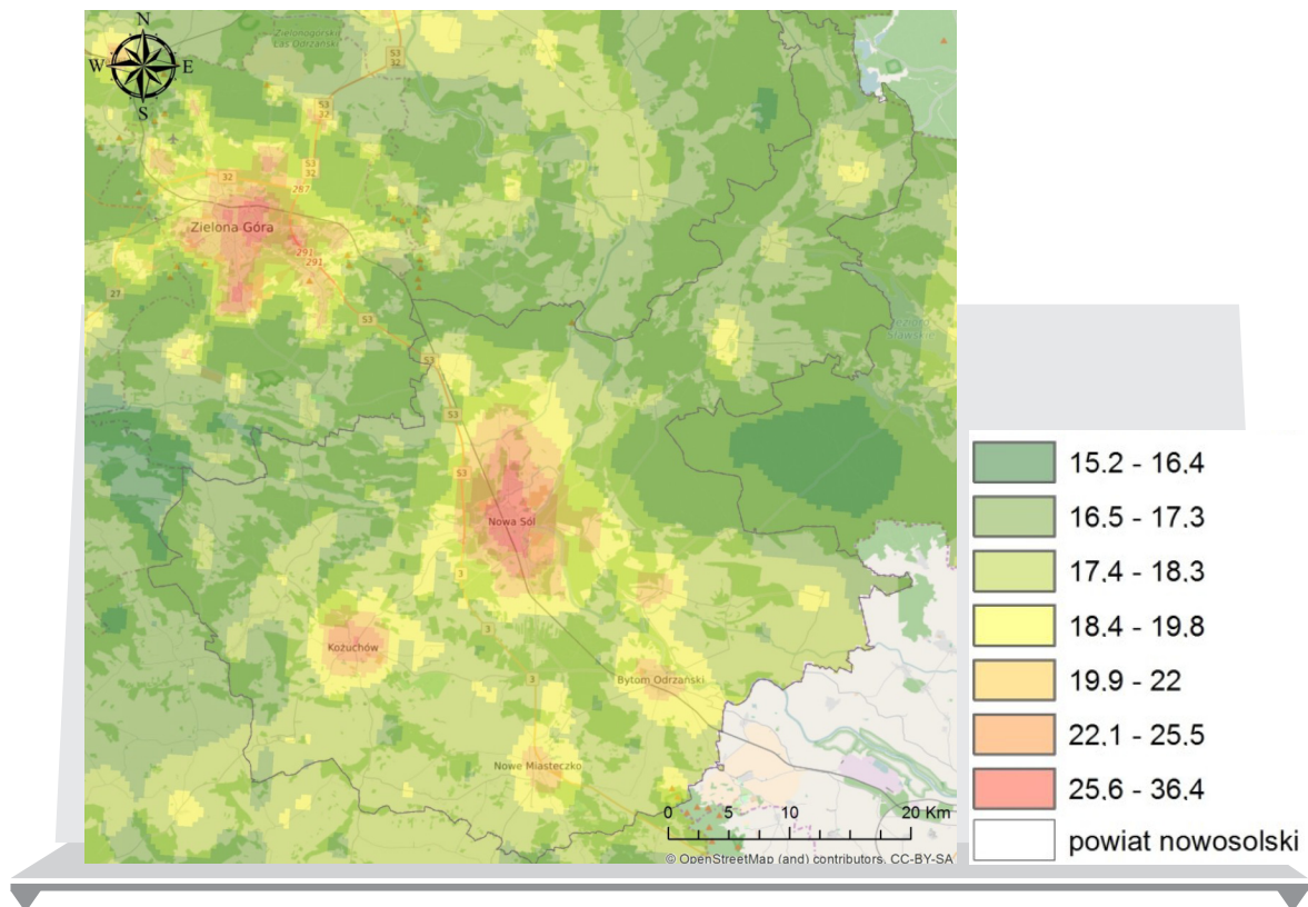
Figure 1. The average annual concentration of PM10 [ \mu\text{g}/\text{m}^3 ] in the Nowa Sól district in 2015
