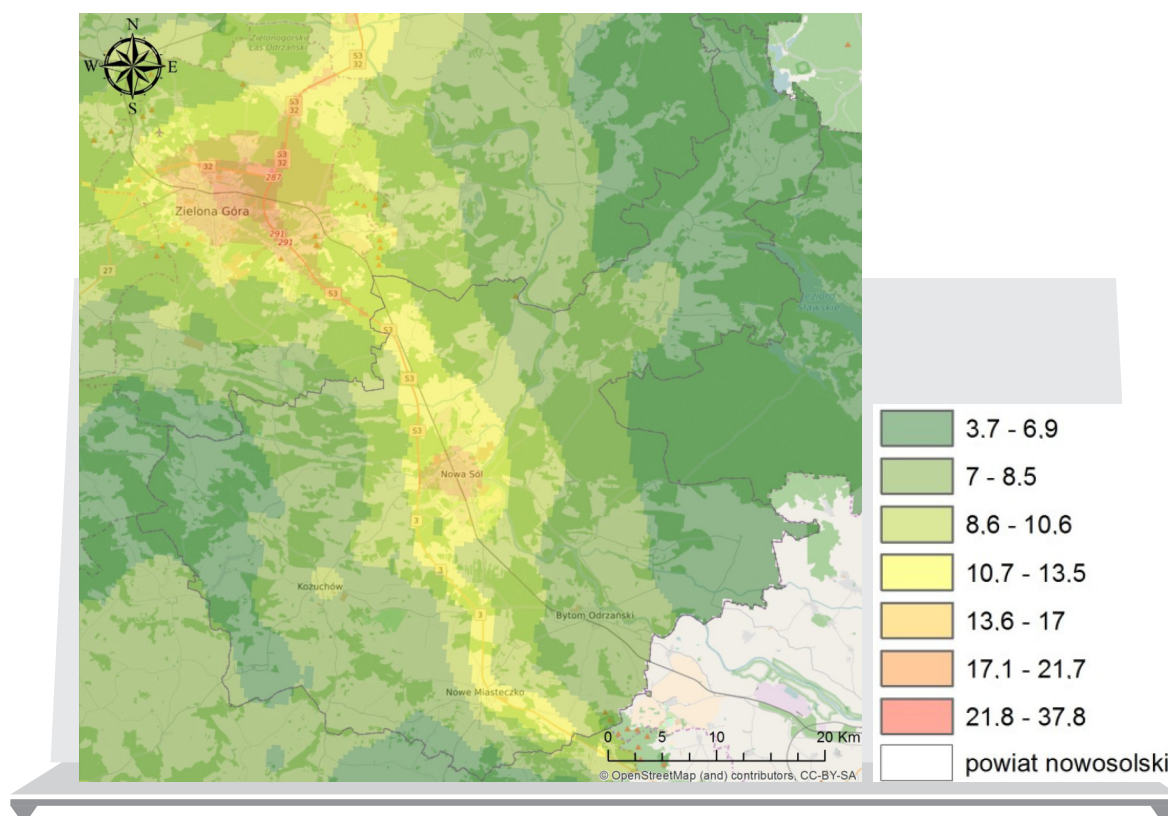
Figure 2. The mean concentration of nitric oxide [ \mu\text{g}/\text{m}^3 ] in the Nowa Sól district in 2015
