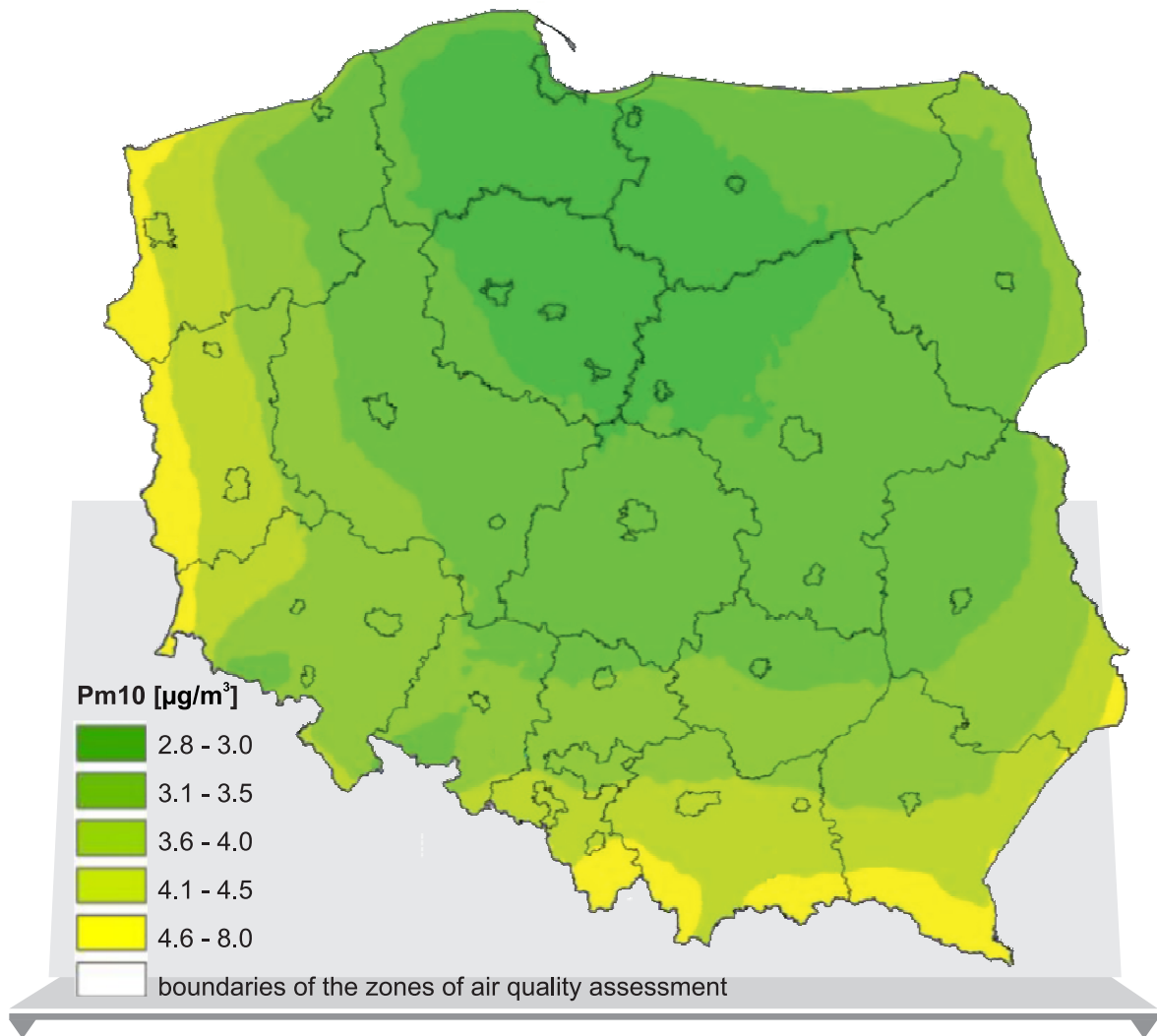
Figure 3. Emissions of PM 10 from neighboring countries in 2015
