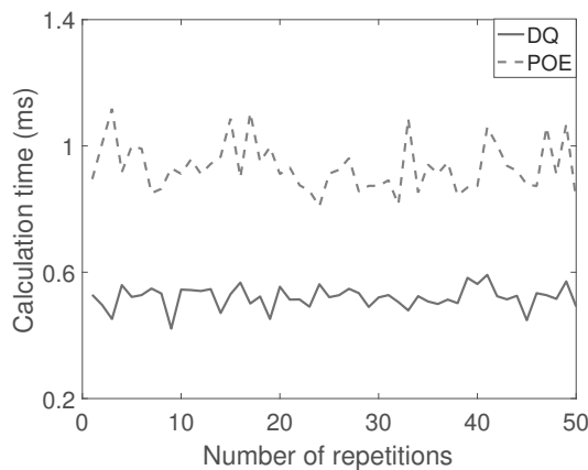
Fig. 9. Comparison of the computation load for the forward kinematics problem (DQ: dual quaternions method, POE: exponential product method).
