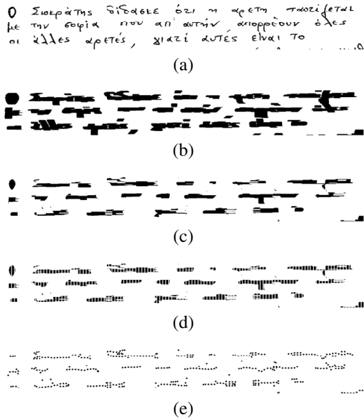
Fig. 7. Pre-processing of the given text into centroids: initial text (a), after dilation (b), after erosion (c), cut image (d), centroid positions (e).
