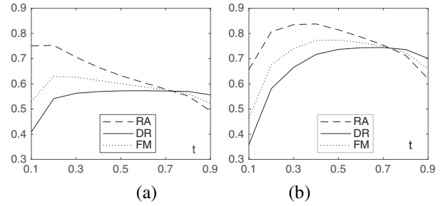
Fig. 10. Results evaluated using the projection algorithm with the border strategy (a) and the center line strategy (b).
