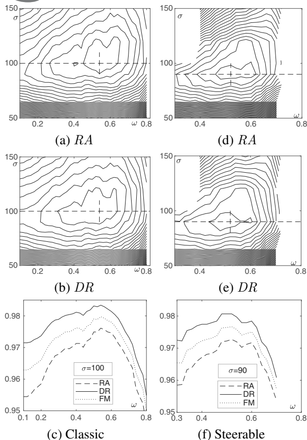
Fig. 11. Results evaluated using TV (original (a)–(c), by steerable filters (d)–(f)), with \omega = 0.1 \div 0.8 and RA for \sigma = 50 \div 150 ((a) and (d)), DR for \sigma = 50 \div 150 ((b) and (e)), profile for \sigma = 100 (c), profile for \sigma = 90 (f).
