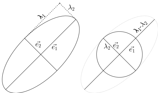
Fig. 4. Tensor decomposition.
