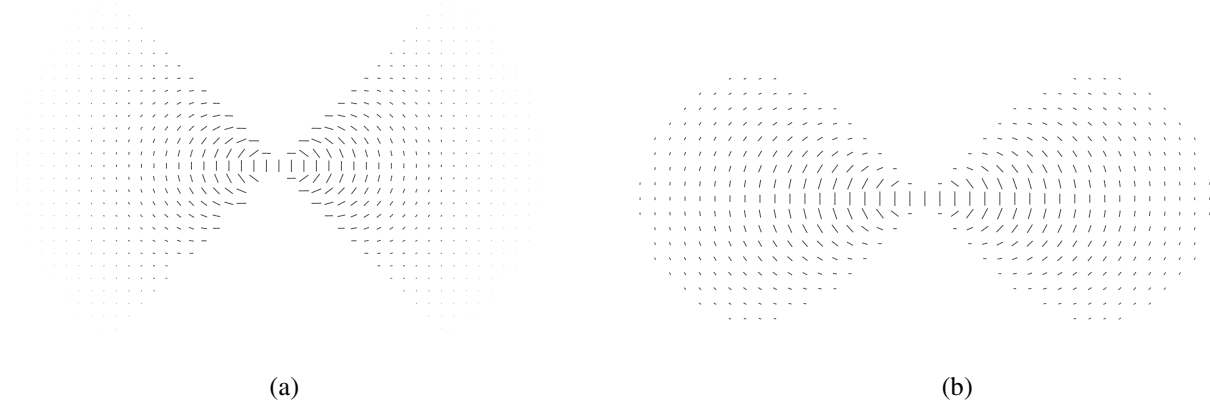
Fig. 6. Voting kernel for original TV (a) and steerable filters (b).
