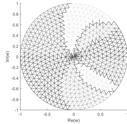
Fig. 4. Final mesh obtained for system S_1 after test execution with \Delta r = 0.1 . Quadrants of the w -plane: ■ Q = 1 , ■ Q = 2 , ■ Q = 3 , ■ Q = 4 .
