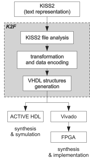
Fig. 4. Typical investigation path based on the K2F tool.
