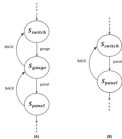
Fig. 5. Example sequence of events.
