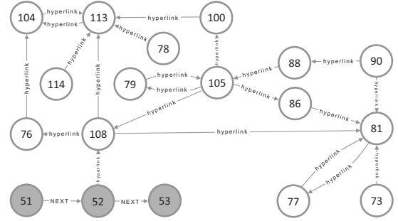
Fig. 6. Transitions between wiki pages accessed from one of the static hyperlinks (108) of PFP command 52.
