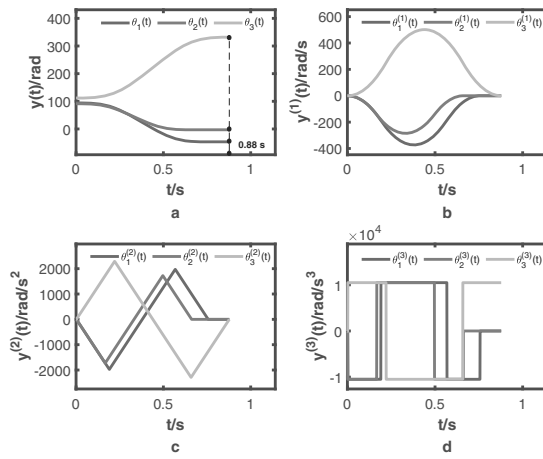
Fig. 5. Time optimal trajectories of three ideal motors of the UVW robot.
