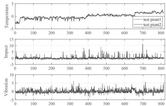
Fig. 8. Data normalization.
