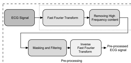
Fig. 3. Pre-processing of the original ECG beat.
