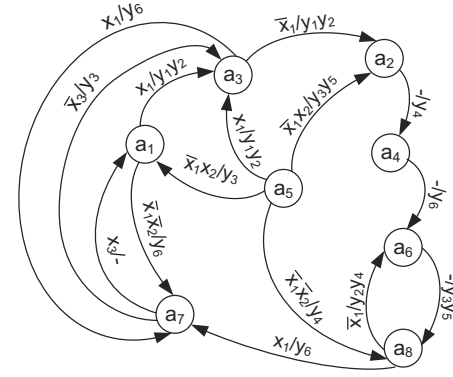
Fig. 1. State transition graph of Mealy FSM A_o .
