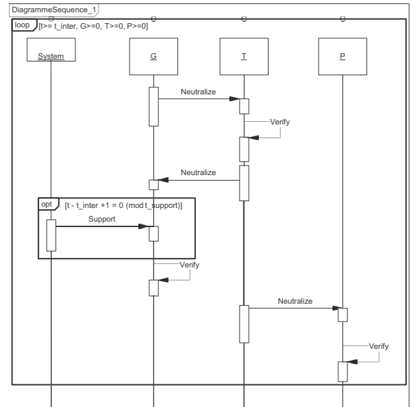
Fig. 5. Sequence diagram of the three steps of the scenario's second phase.
