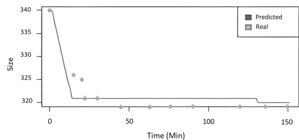
Fig. 7. Real and predicted size of a population (BA).
