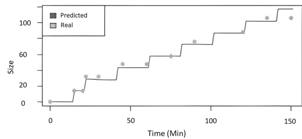
Fig. 6. Real and predicted size of government forces (BA).
