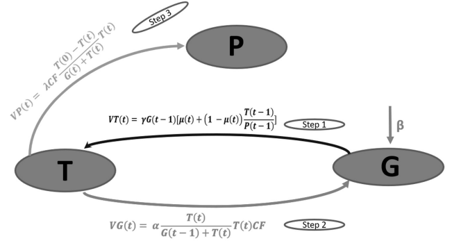
Fig. 4. Three steps of the scenario's second phase.
