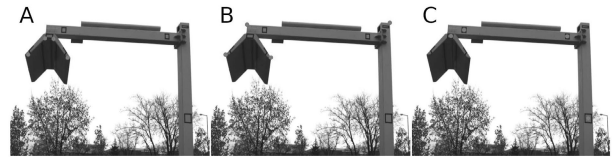
Fig. 8. Location of keypoints for charger pose estimation: four points located on the head and called head (a), four points located on the natural corners of the head and the mast, called corners (b), and four points located inside the artificial markers, called markers (c).
