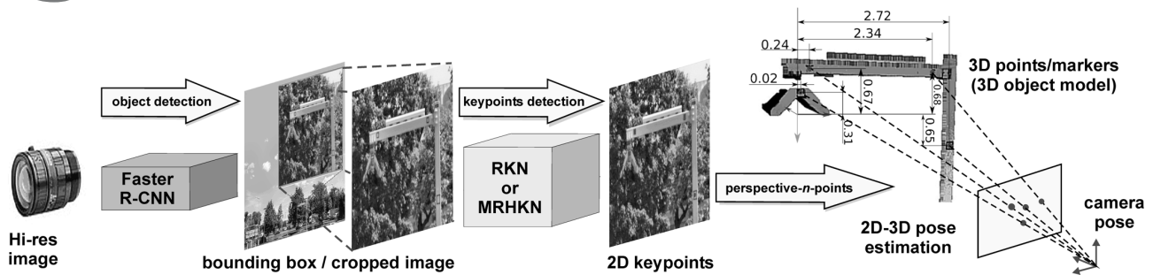
Fig. 2. Block diagram of the image processing and pose estimation pipeline used for positioning of electric buses with respect to a charging station. The CAD model is a visualization of the 3D mesh obtained from SURPHASER 100HSX with annotated dimensions between markers.
