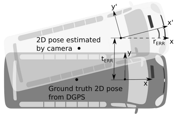
Fig. 11. Vision-based localization system is evaluated with respect to the translation error on the ground plane (2D position) and the orientation error (yaw) understood as the difference between the estimated and the ground truth headings of the bus.
