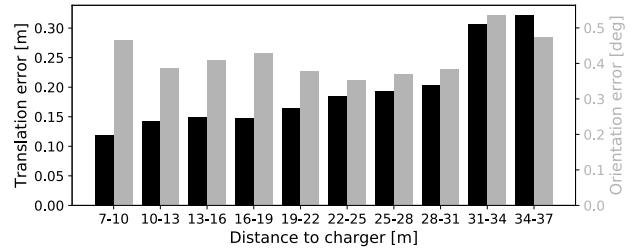
Fig. A1. Distribution of the translation error (black bars) and orientation error (gray bars) as a function of the distance to the charging station for MRHKN + markers .
