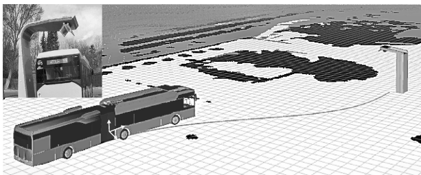
Fig. 1. Illustration of the docking maneuver with an articulated bus. The visualized coordinate system's origin is coincident with the guidance point, while the curved line indicates the planned trajectory. The inset image shows a charging station with example salient features, as seen by the localization system's camera.
