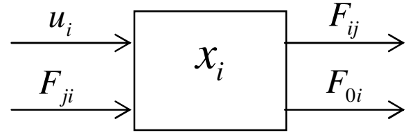
Fig. 1. Compartmental system: i -th subsystem.
