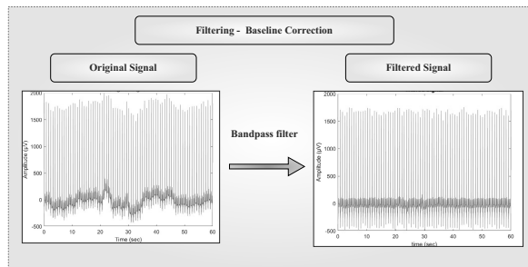
Fig. 2. Filtering of the ECG signal for baseline correction.
