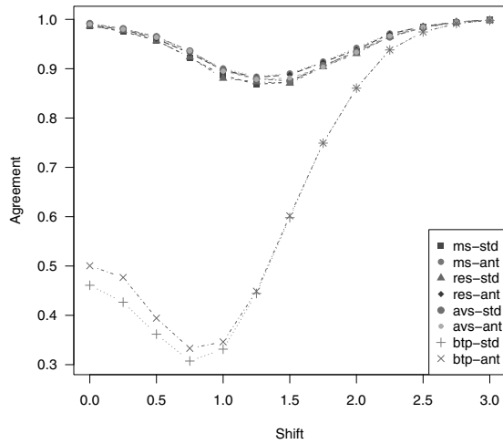
Fig. 2. Simulated ACC values for the KS test, X \sim \mathbb{F}_{(N,U,U)} , and K = 10, n = m = 10 (shift added to Y ).
