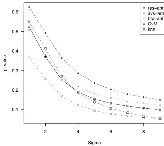
Fig. 12. Estimated p -values, X \sim \mathbb{F}_{(N,U,U)} , and K = 10, n = m = 10 (increasing \sigma ), averaged p -values: CvM test based approaches.
