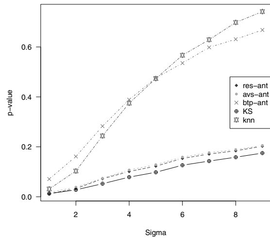
Fig. 13. Estimated power, X \sim \mathbb{F}_{(N,U,U)} , and K = 10, n = m = 10 (increasing \sigma ), averaged p -values: KS test based approaches.
