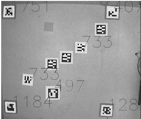
Fig. 19. AR recognition. The one color-painted point on a capture describes the start point—the robot's actual position.
