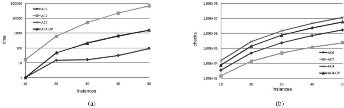
Fig. 2. Behavior of AC6, AC7, AC4 and AC4-OP on different instances of the pigeon problem: runtime [ms] (a), number of constraint checks (b).
