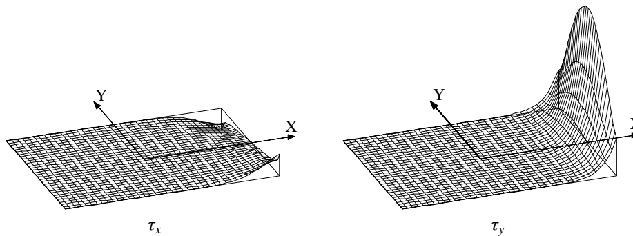
Fig. 15. The base function (\tau_x, \tau_y)_{e12}
