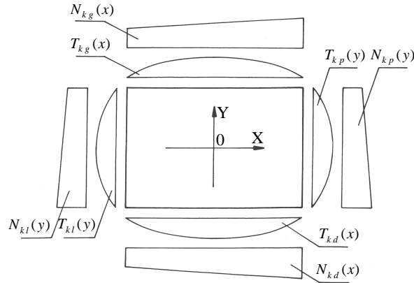
Fig. 3. Schematic graphs of the functions T_{kg}, N_{kg}, T_{kp}, N_{kp}, T_{kd}, N_{kd}, T_{kl}, N_{kl}
