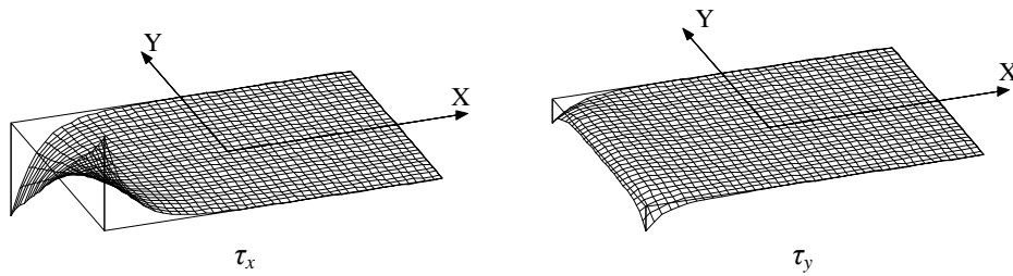
Fig. 11. The base function (\tau_x, \tau_y)_{e8}
