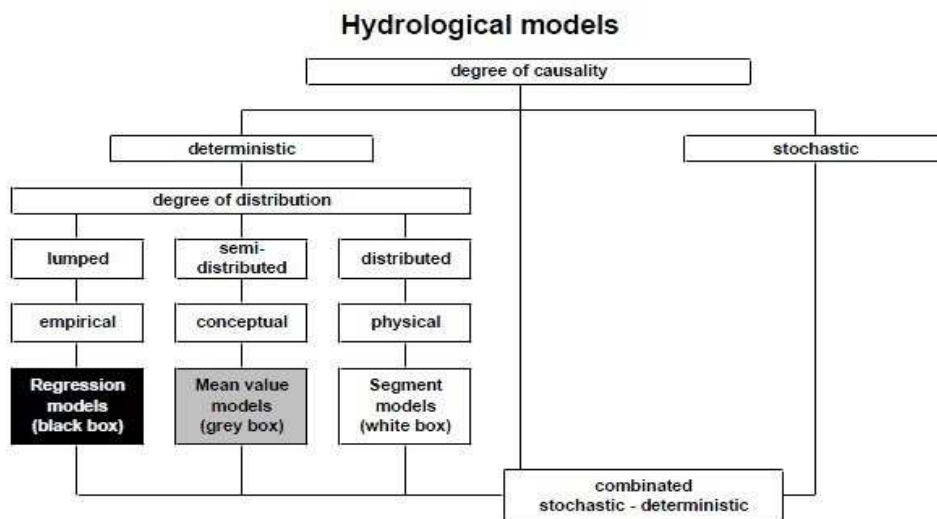
Fig. 3. Illustrative classification of hydrological models [21]
