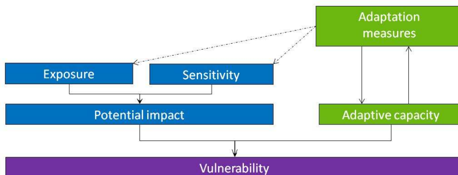
Fig. 1. Vulnerability of socio-ecological system to flood risk adapted from [1] after [2]
