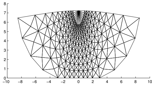
Fig. 9. Hertz test: Adapted mesh (Deformed configuration).
