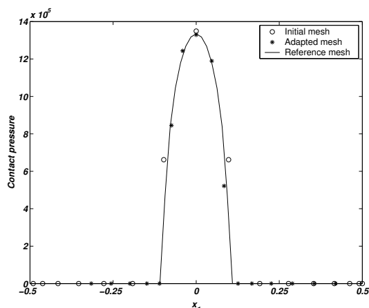
Fig. 13. Disc test: Comparison of contact pressures.
