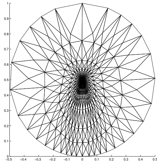
Fig. 12. Disc test: Adapted mesh.
