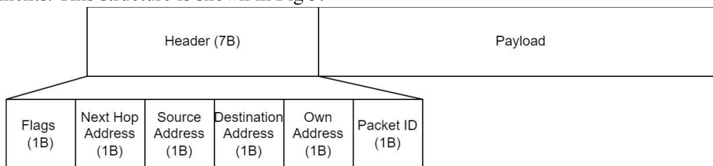
Fig. 3. Packet structure of Kangaroo protocol stack. Rys. 3. Struktura pakietu stosu protokołów Kangaroo.
