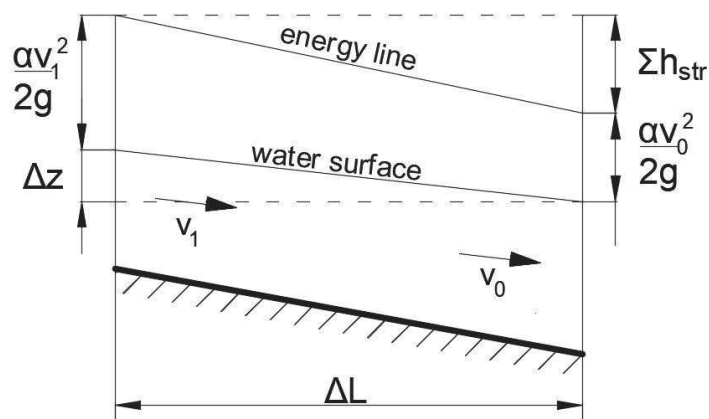
Fig. 1. The section of river contained between two cross-sections [3]
