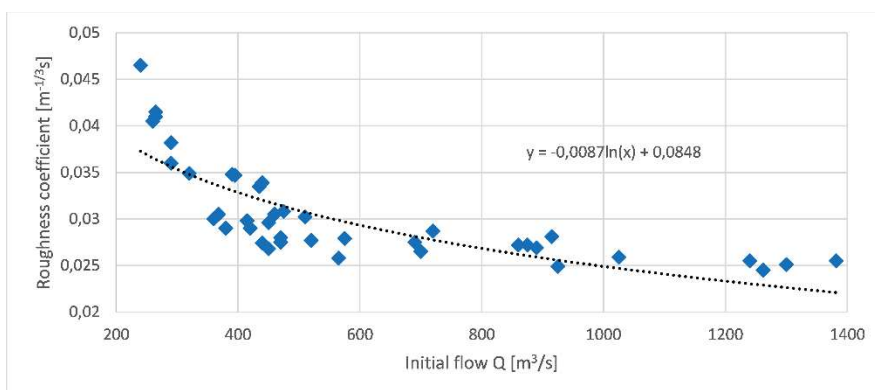
Fig. 2. Changes in Manning roughness as a function of the input flow by Kurnatowski [4,5]
