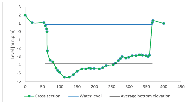
Fig. 3. Cross-section bathymetry
