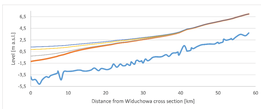
Fig. 4. Backwater curves for SSQ flows. Light blue – river bottom; orange – normal depth (without damming); grey - curve for Q = 599 \text{ m}^3/\text{s} and W = -0.275 \text{ m. a.s.l.} ; gold - curve for Q = 599 \text{ m}^3/\text{s} and W = 0.855 \text{ m. a.s.l.} ; blue - curve for Q = 599 \text{ m}^3/\text{s} and W = 1.292 \text{ m. a.s.l.}
