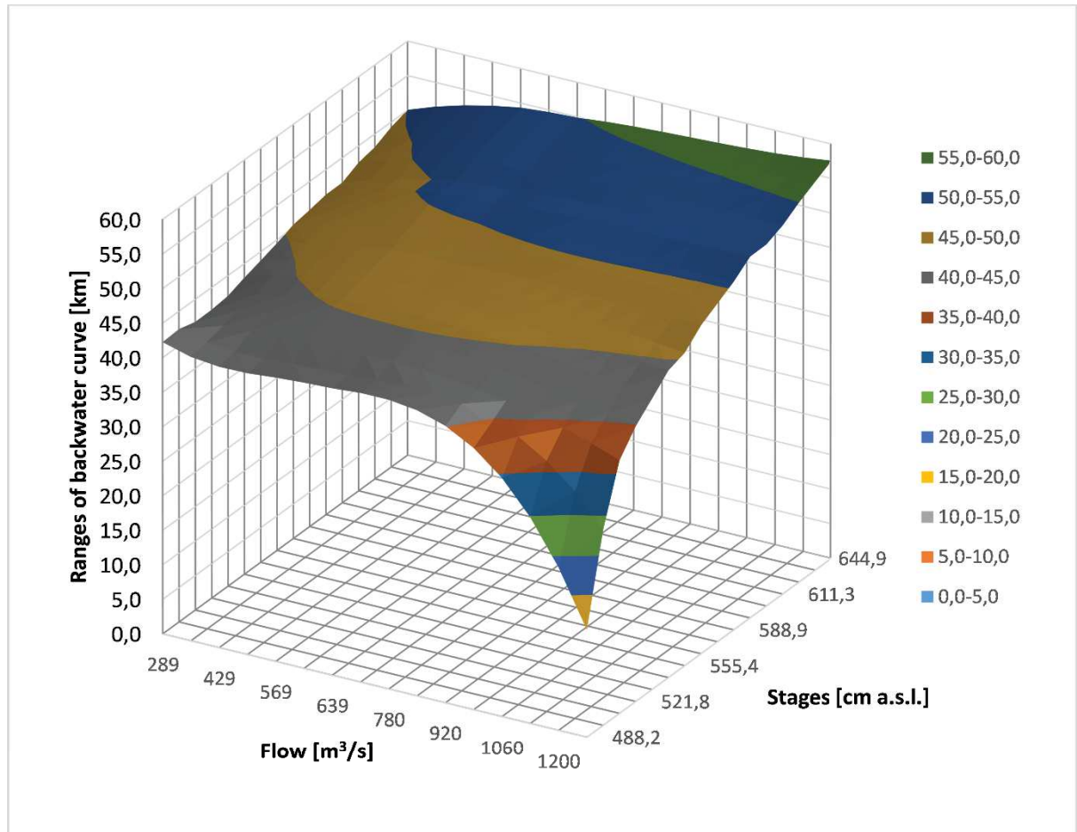
Fig. 5. Calculated ranges of backwater curves at various boundary conditions
