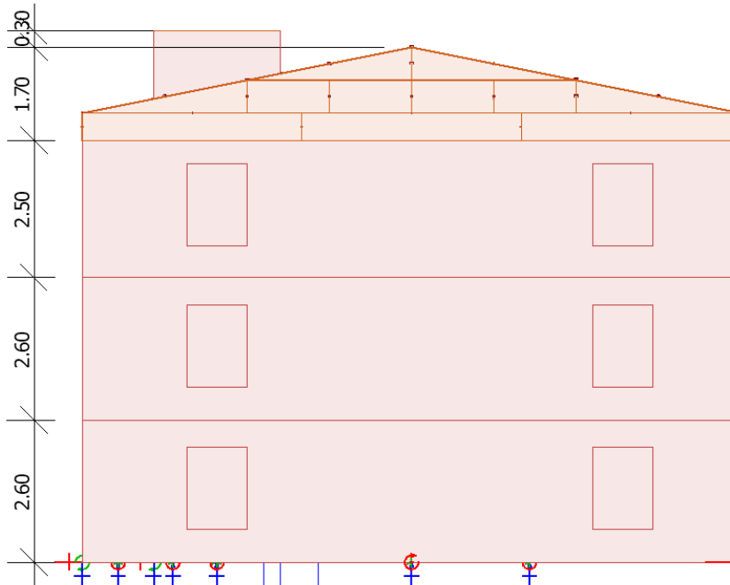
Fig.5. Facade towards X- (unit: m ).
