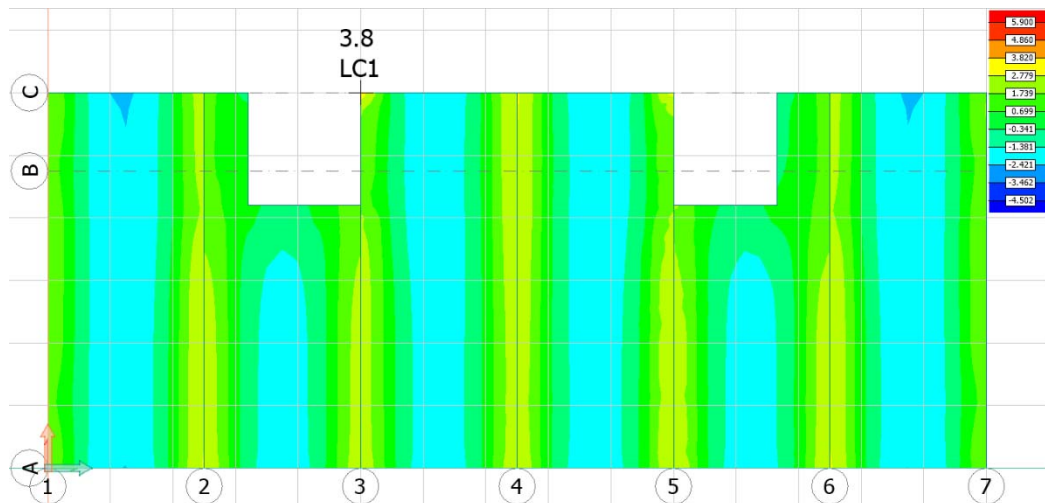
Fig.10. Stress distribution in slabs of storey I, Sigma X-top (unit: MPa).
