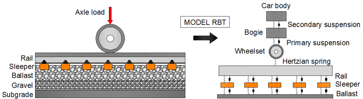
Fig.2. Scheme of relations between track-bridge-rolling stock.
