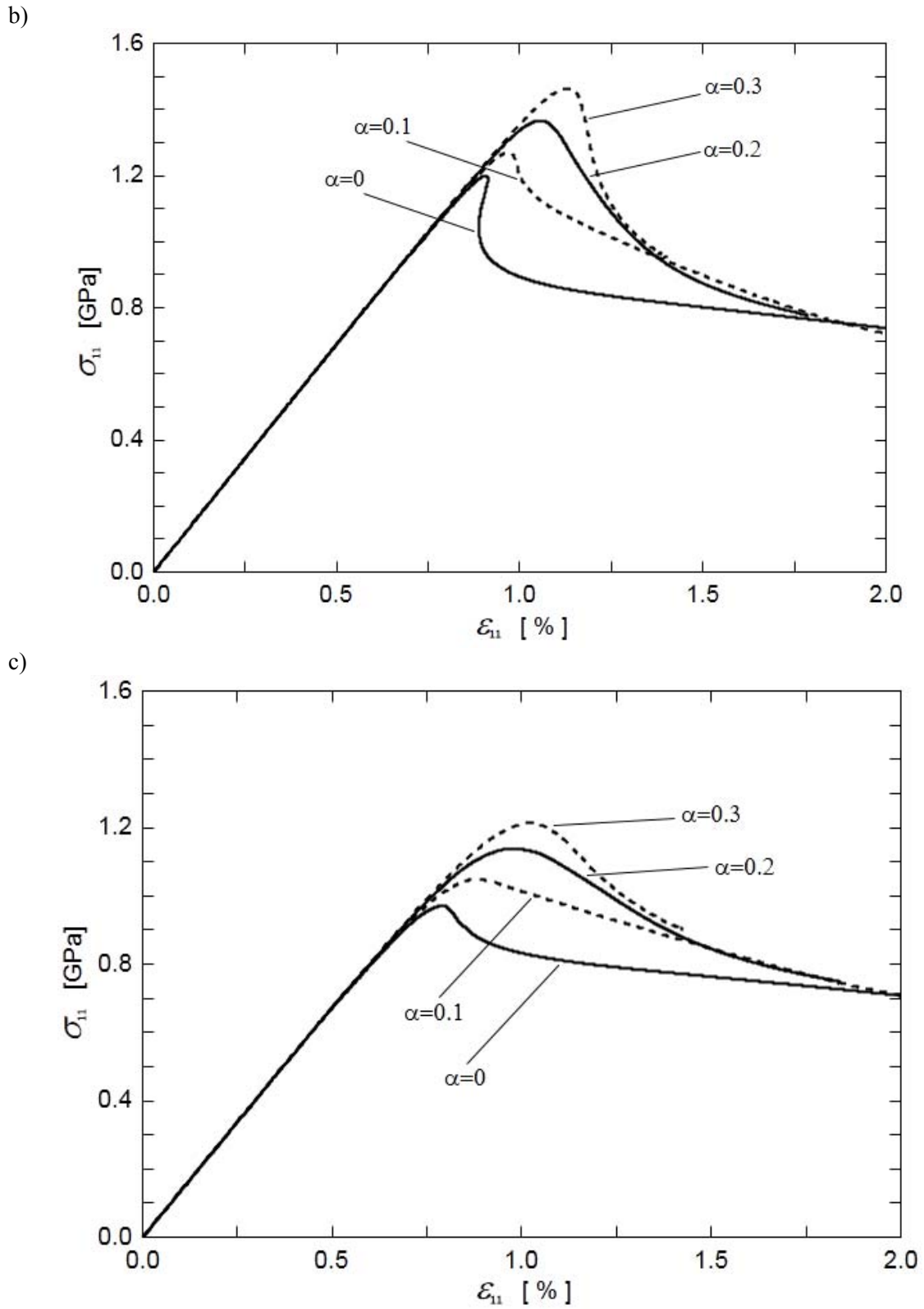
Fig.3. Prediction of the compressive stress–strain curves for various values of the pressure sensitivity factor \alpha . Responses for (a) \Theta = 1.71^\circ ; (b) \Theta = 2.40^\circ ; (c) \Theta = 3.42^\circ .
