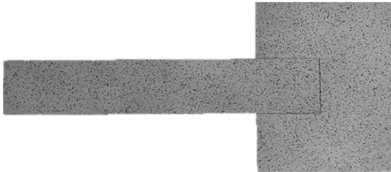
Fig.6 The stochastic layer on tested set.
