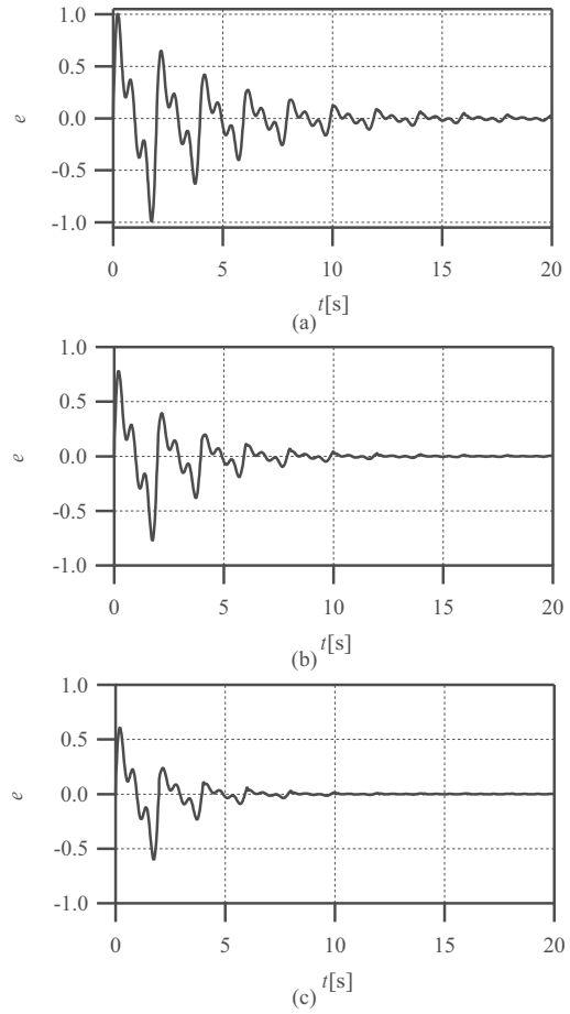
Fig. 4. Tracking error for the parameter sets (40): \alpha = 0.1, \beta = 0.01 (a), \alpha = 0.1, \beta = 0.43 (b), \alpha = 0.8, \beta = 0.43 (c).
