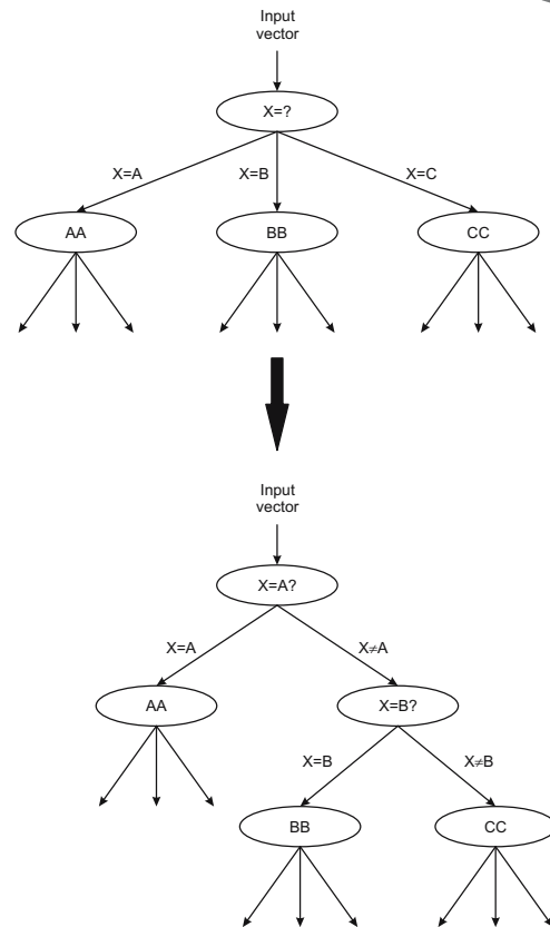
Fig. 3. Example of transformation of a third-order node into an equivalent binary subtree.
