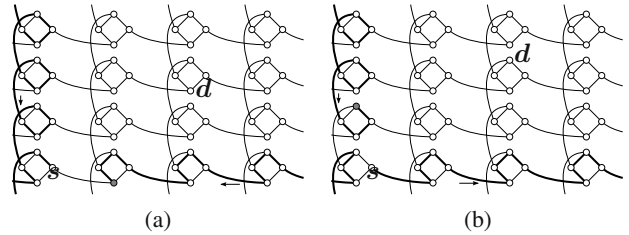
Fig. 10. Step 1: path initialization for vertical (a) and horizontal (b) traversals. Newly selected edges in bold; the greyed node is the head of the (still in construction) path.
