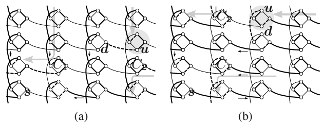
Fig. 12. Step 8: going through C_1 and C_2 before reaching C(u) and eventually d in the case of vertical (a) and horizontal (b) traversals. Newly selected edges in dashes.
