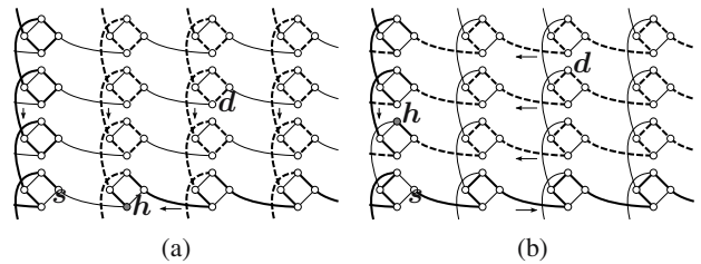
Fig. 11. Step 2: path extension for vertical (a) and horizontal (b) traversals. Newly selected edges in dashes.
