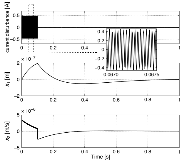
Fig. 8. Responses of the system states to a high frequency sinusoidal disturbance of the control current.
