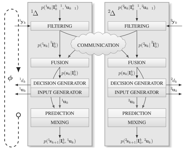
Fig. 9. Scheme of the distributed AFD algorithm.
