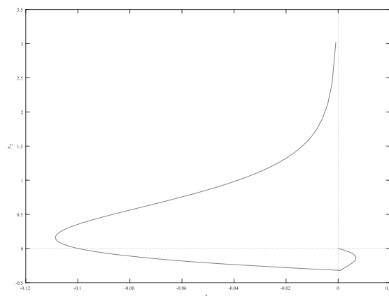
Fig. 1. Time-optimal phase trajectory of (46), (47) for \alpha = 0.7 , x_1^0 = 0 , x_2^0 = 1 .
