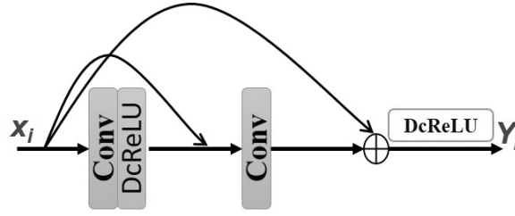
Fig. 3. Building block of the modified residual dense block (MRDB).
