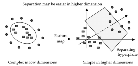
Fig. 4. Kernel function mapping from input data to a richer feature space.
