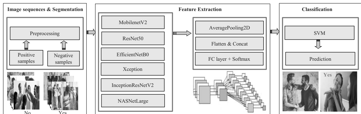
Fig. 2. Estimating cyberbullying with the proposed model.
