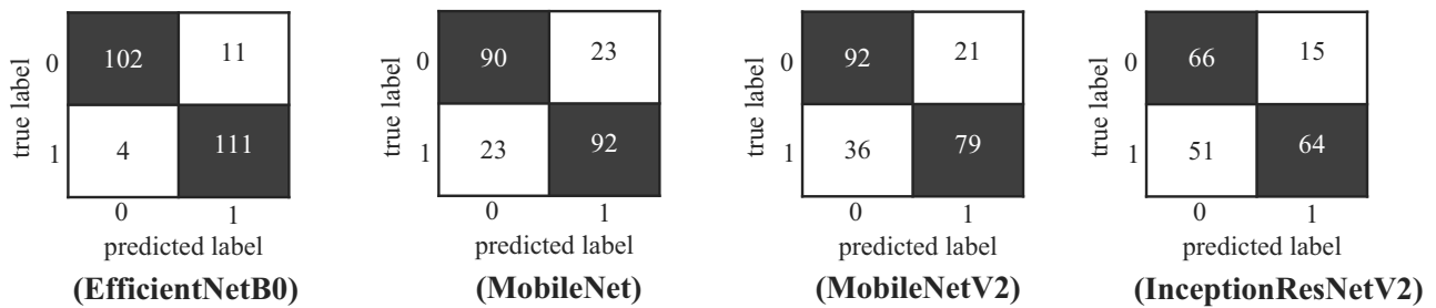
Fig. 7. Confusion matrix for EfficientNetB0, MobileNet, MobileNetV2 and InceptionResNetV2 models.
