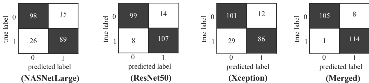
Fig. 8. Confusion matrix for NASNetLarge, ResNet50, Xception and Merged + Softmax.
