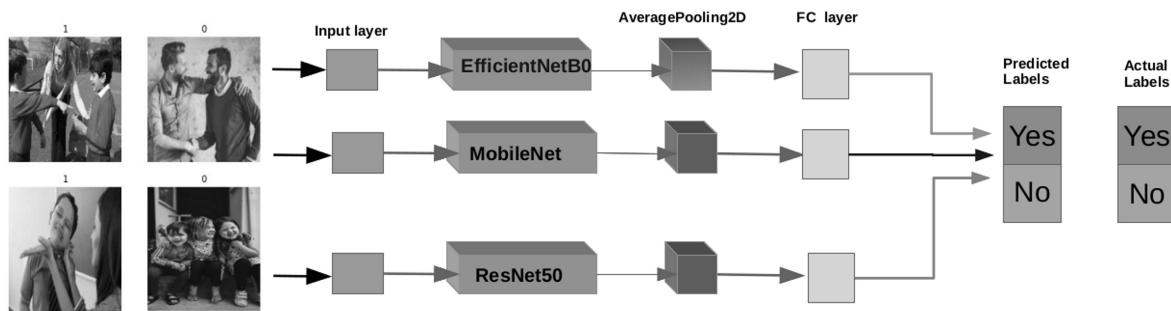
Fig. 1. Estimating cyberbullying with the CNN model.
