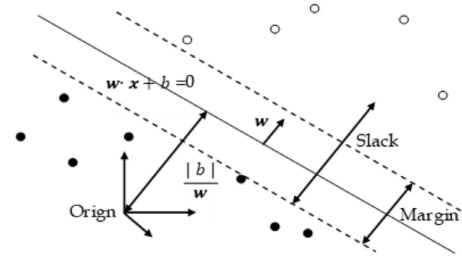
Fig. 3. Hyperplane margin.
