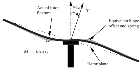
Fig. 5. Propeller flapping approximation.
