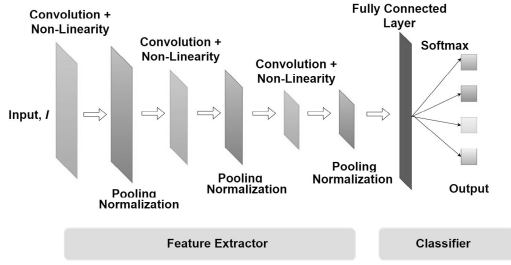
Fig. 2. Typical CNN architecture.
