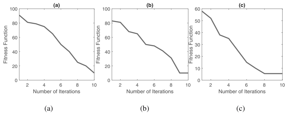
Fig. 12. Fitness value for each iteration using two convolutional layers (a), three convolutional layers (b) and four convolutional layers (c) of the CNN.
