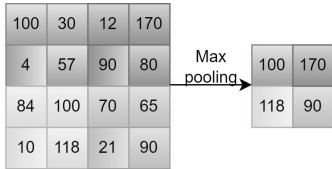
Fig. 4. Diagrammatic illustration of 2 \times 2 max-pooling.
