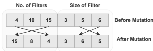
Fig. 9. Mutation.
